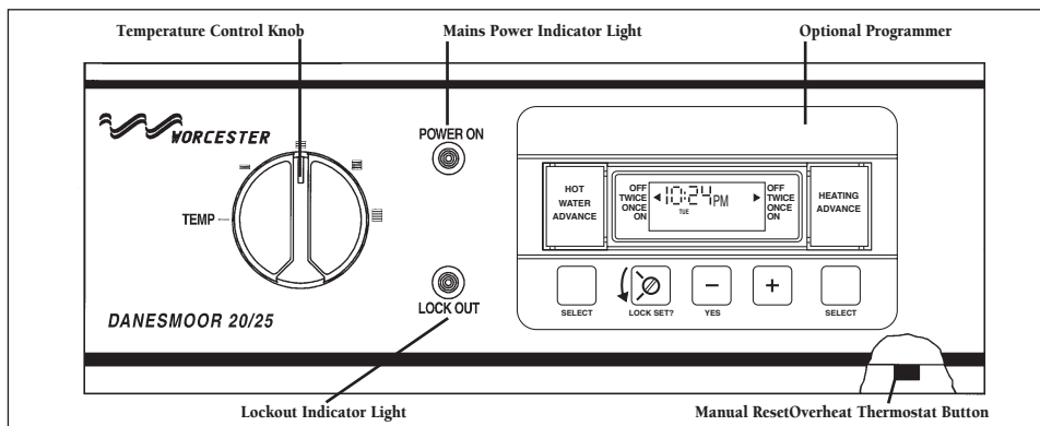
Fig. 1. Control Facia
